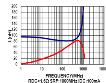
MHI0402D82NJT
