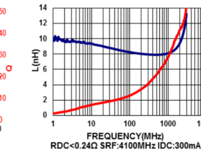
MHI0402D8N2JT
