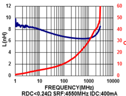
MHI0402D6N8JT
