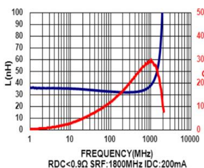
MHI0402D33NJT
