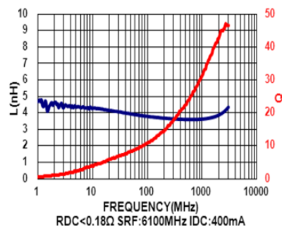
MHI0402D3N9ST
