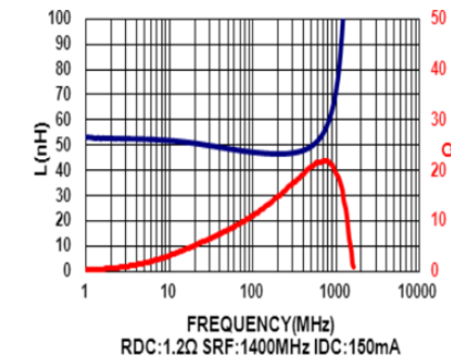
MHI0402D47NJT
