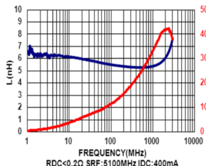
MHI0402D5N6ST
