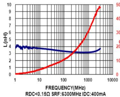
MHI0402D3N3ST
