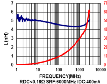
MHI0402D4N7ST
